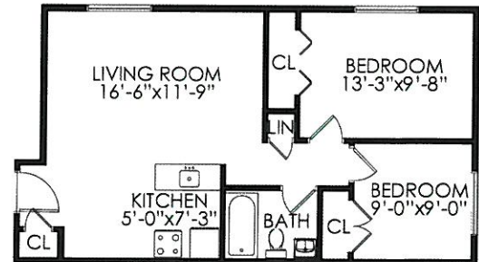
TWO BEDROOM 679 SQ. FT.
